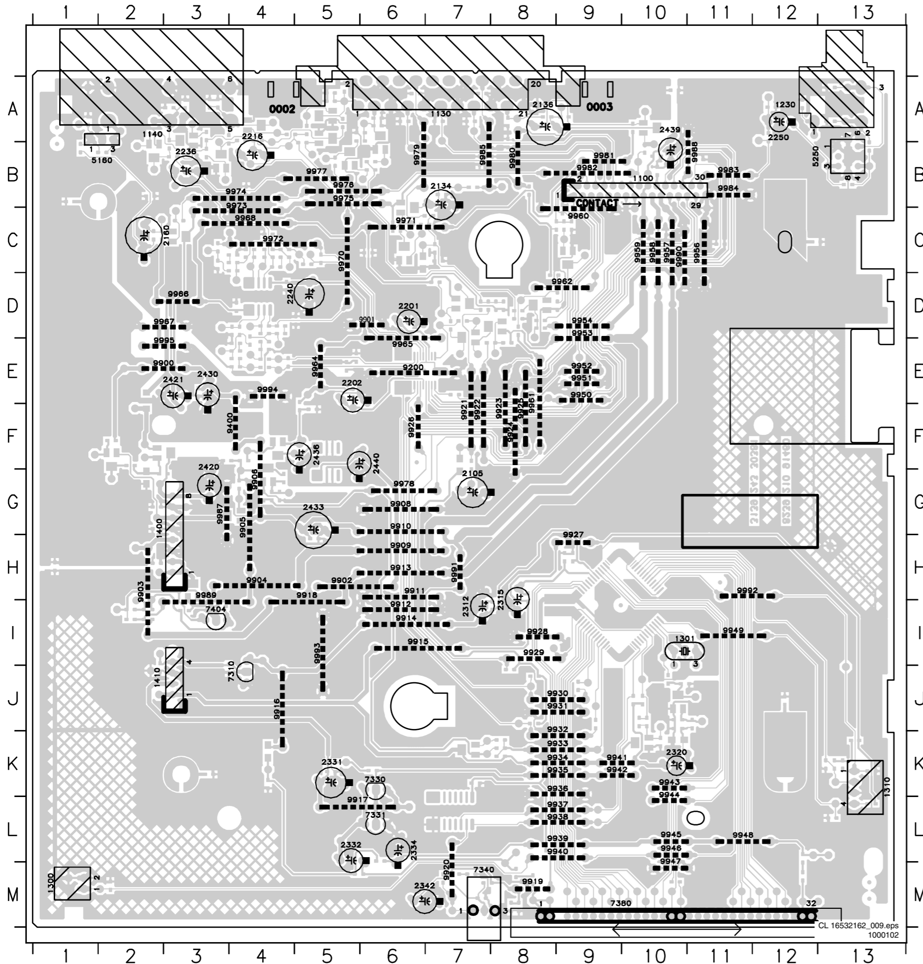
Layout Motherboard (Top View)
